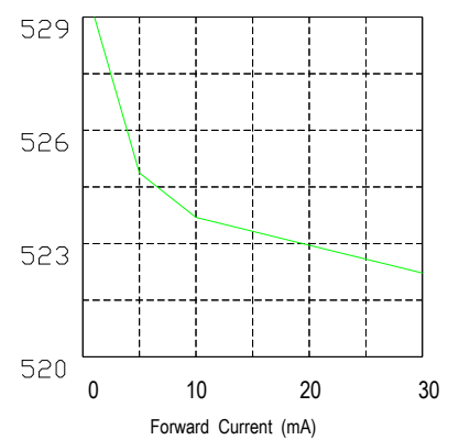
Forward Current vs. Dominant wavelength (Ta=25°C)
