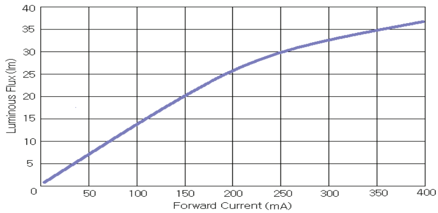
Luminous Flux vs Forward Current
