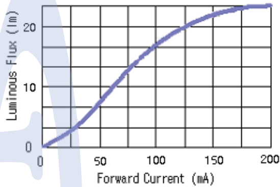
Luminous Flux vs Forward Current
