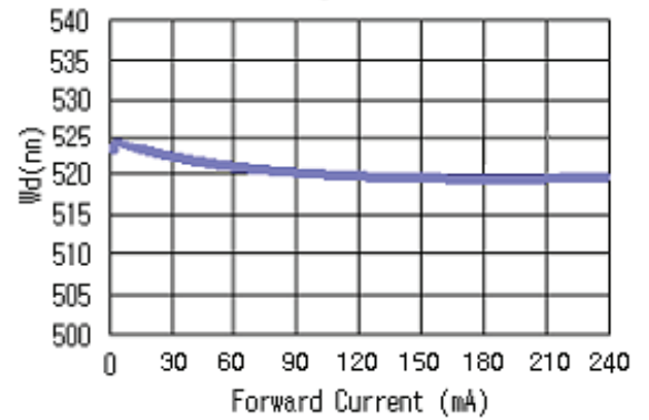
Dominant Wavelength vs Forward Current
