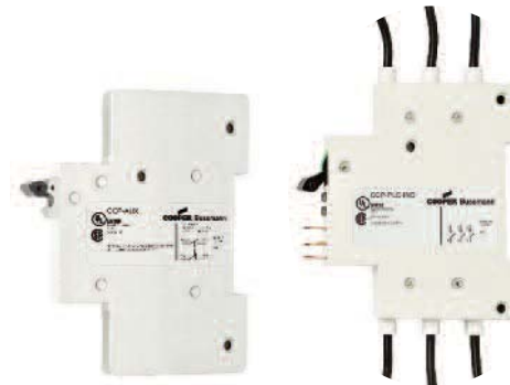
Auxiliary Contacts
