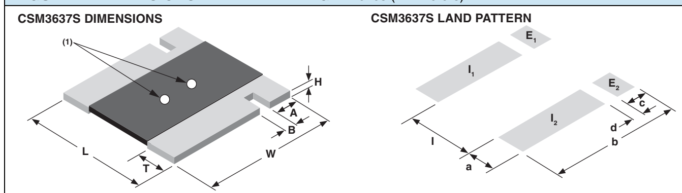
DIMENSIONS - TOLERANCES ± 0.010 (± 0.254)
