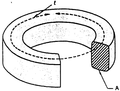
CORE DIMENSIONS (mm) Fig. 1
