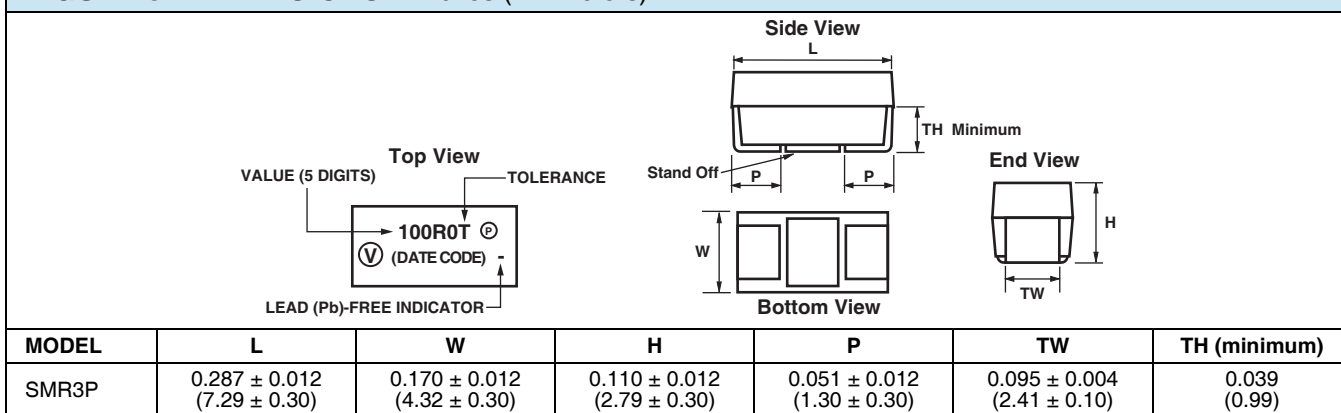
FIGURE 5 - DIMENSIONS in inches (millimeters)
