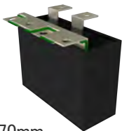
98x38x70mm 400V-200 \mu F (28mm Pitch) Actual Value: 4.1nH (Simulation: 2.5nH)
