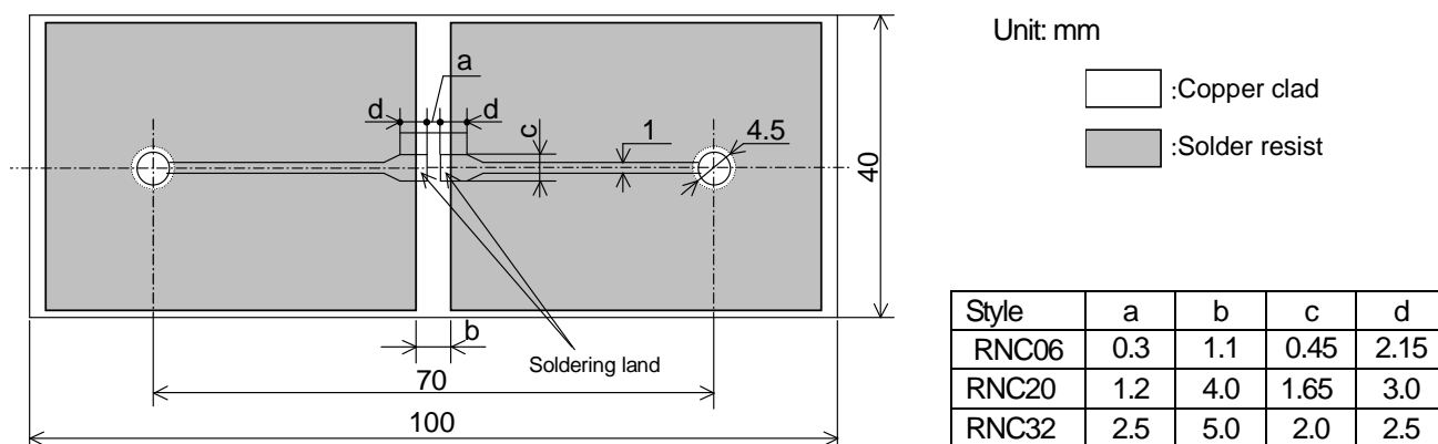
RNC BOUND STRENGTH OF THE END FACE PLATING TEST TEST SUBSTRATE
