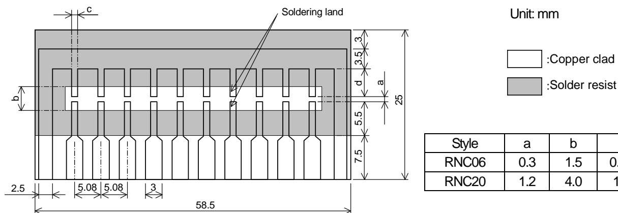
RNC06, 20 TEST SUBSTRATE
