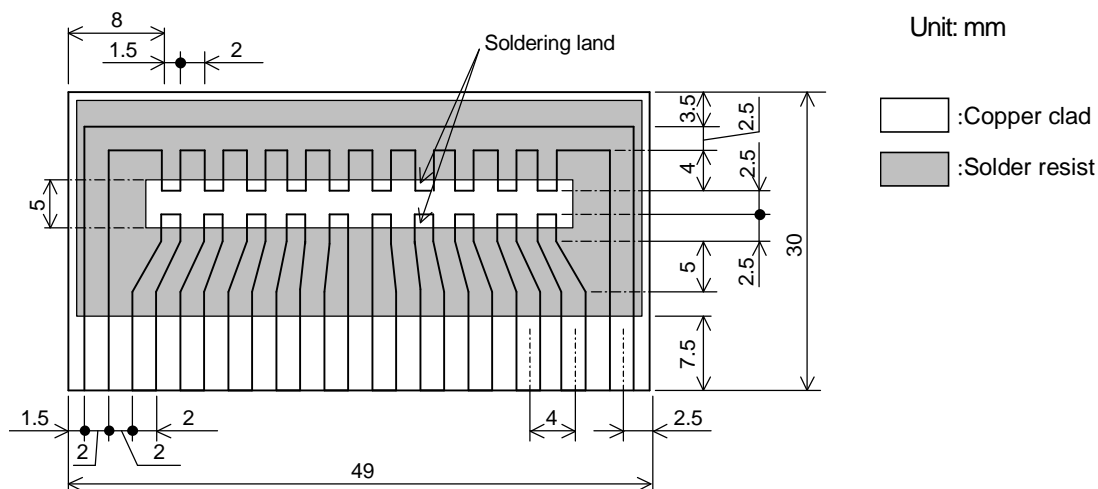
RNC32 TEST SUBSTRATE
